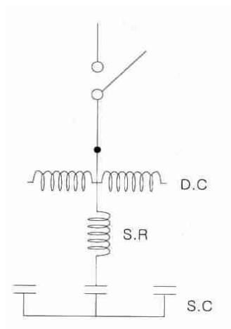
< Discharge coil with internal reactor >
