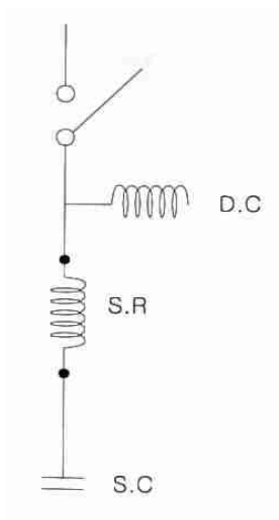
< Normal Discharge Coil >
